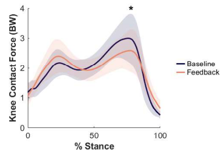
Figure 1: Mean (line) and standard deviation (shaded region) of simulated knee contact force. Feedback to reduce gastrocnemius activity reduced the second peak of knee contact force by 12% ( 0.38 \pm 0.47 BW, *p=0.01 ).
